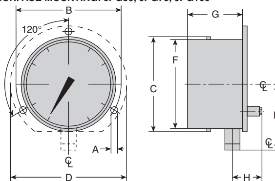
SURFACE MOUNTING: 6PG50, 6PG75, 6PG100
